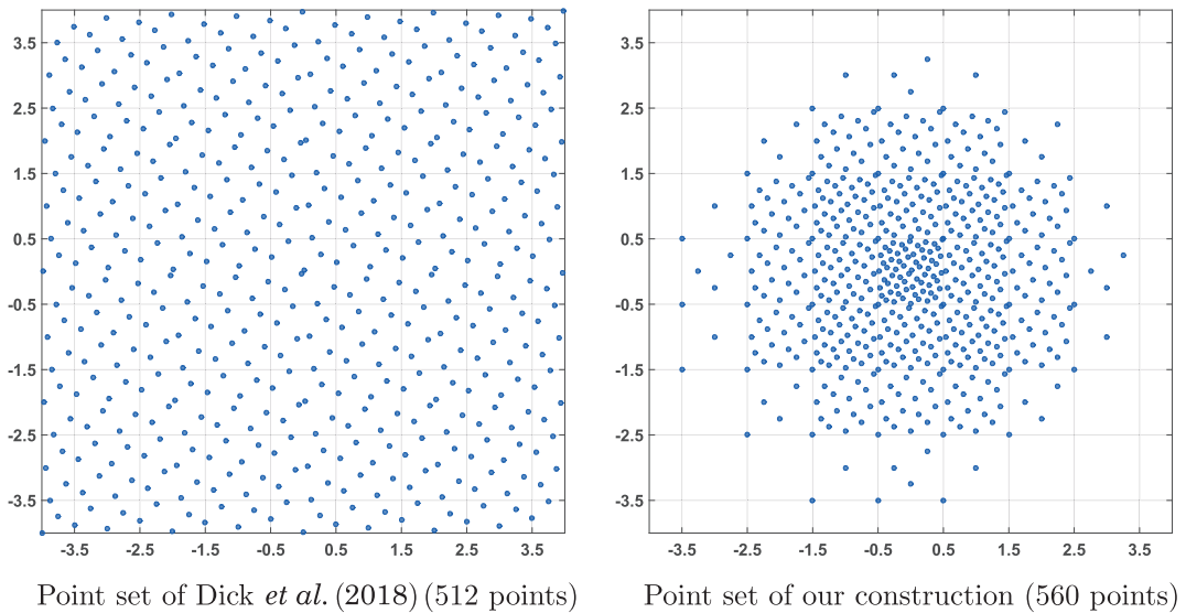
FIG. 1. Distribution of integration nodes in Dick et al. (2018) and in this paper.
