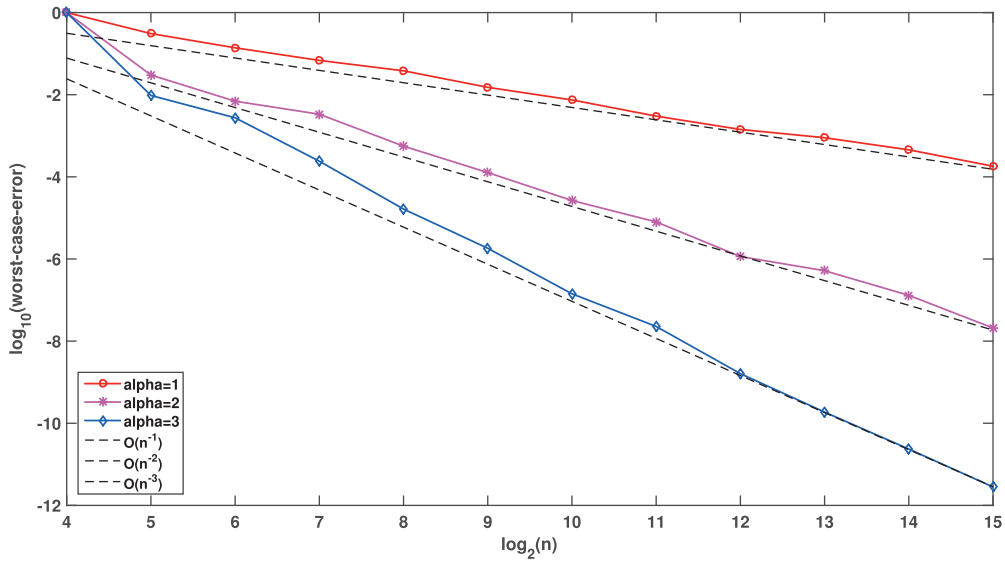
FIG. 2. Errors of the assembling quadratures.
