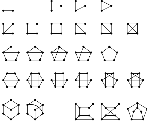
FIGURE 2. The list of all one-dimensional simplicial complexes with vanishing T^2 .
